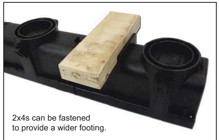
Each channel has four (4) drainage ports that will accept 3" or 4" SCHD 40 or SDR 35 pipe.
